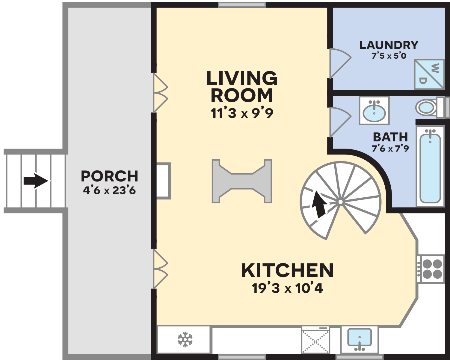
1ST FLOOR
