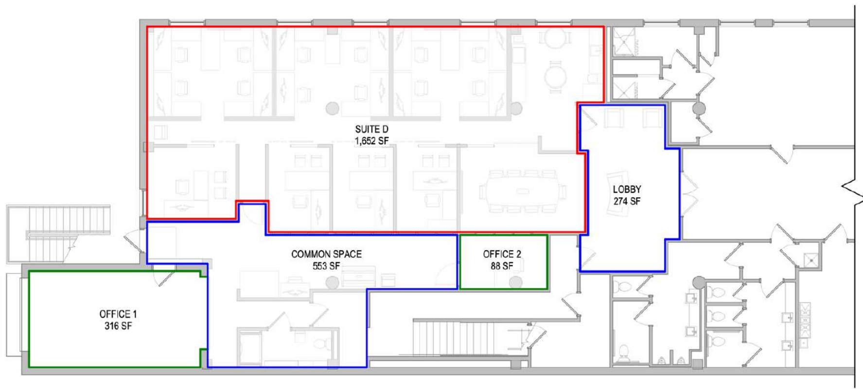
1 FLOOR PLAN - LEVEL 1 A504 1/8" = 1'-0"
