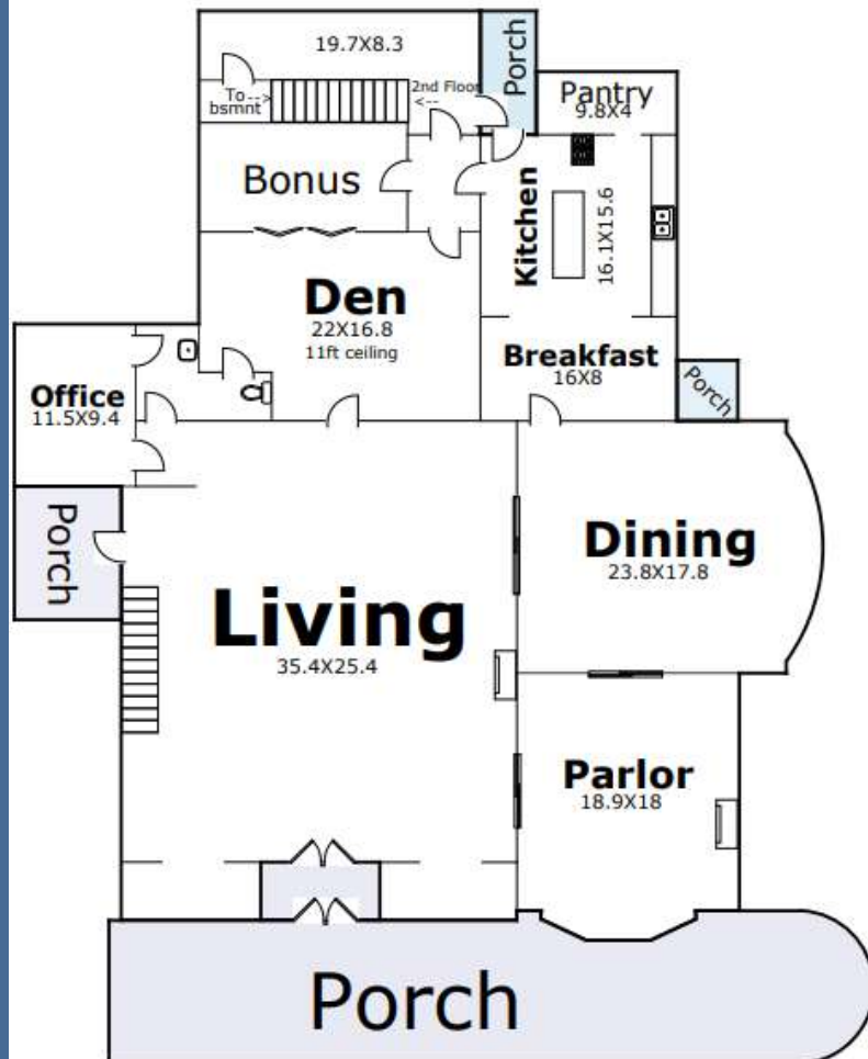
First Floor 13ft ceiling
