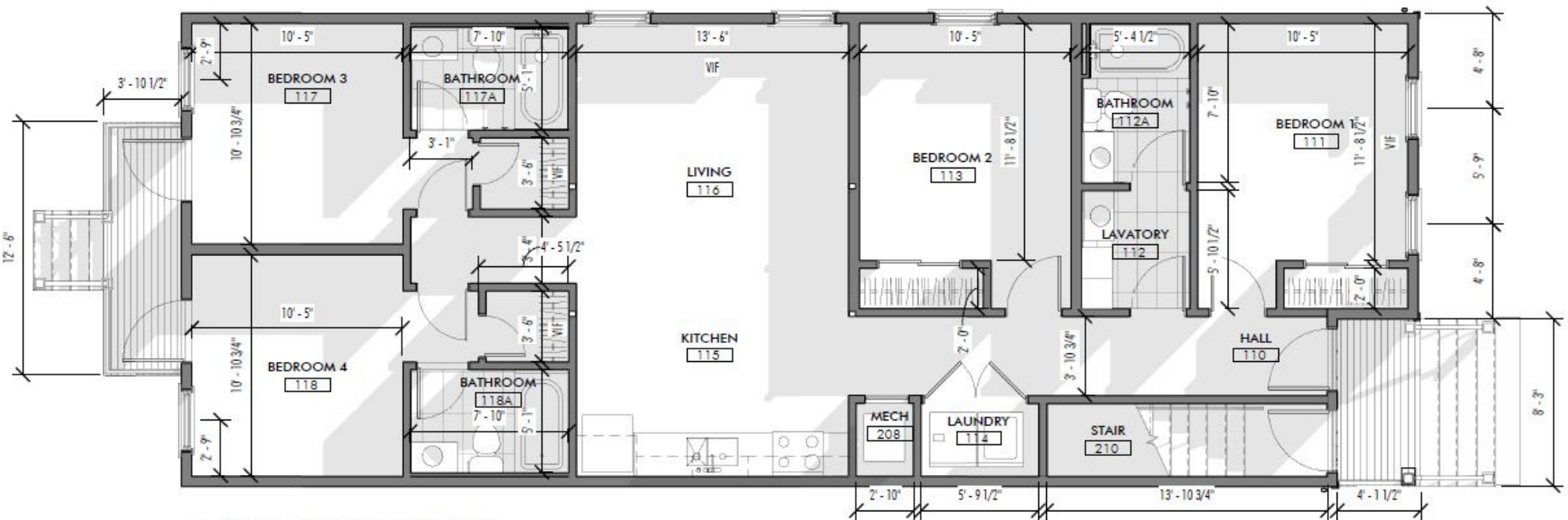
1 FIRST FLOOR PLAN - 2812 PHILIP
