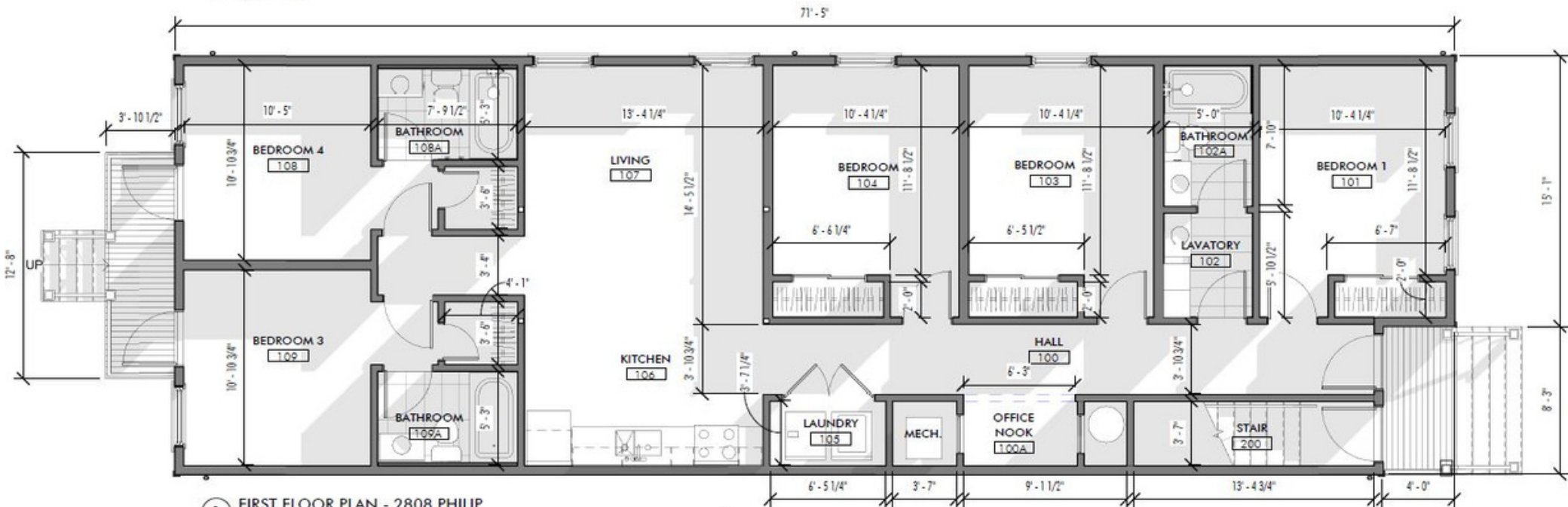
1 FIRST FLOOR PLAN - 2808 PHILIP 3/16" = 1'-0"
