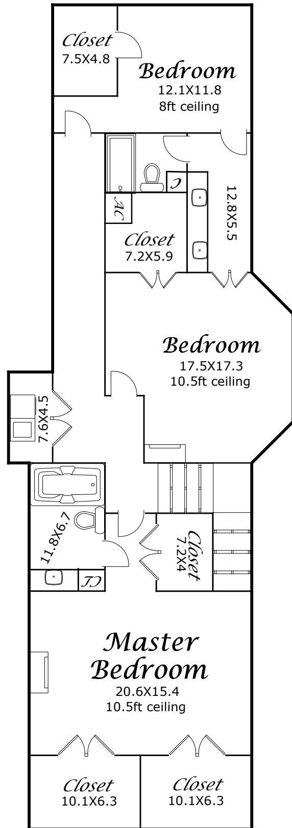
Second Floor
